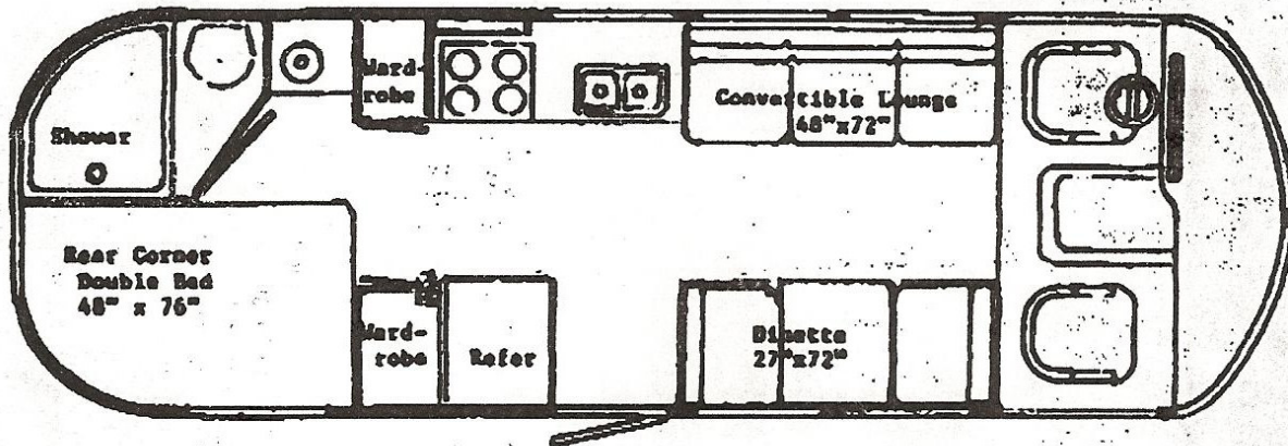
250 AIRSTREAM MOTORHOME - REAR CORNER DOUBLE
